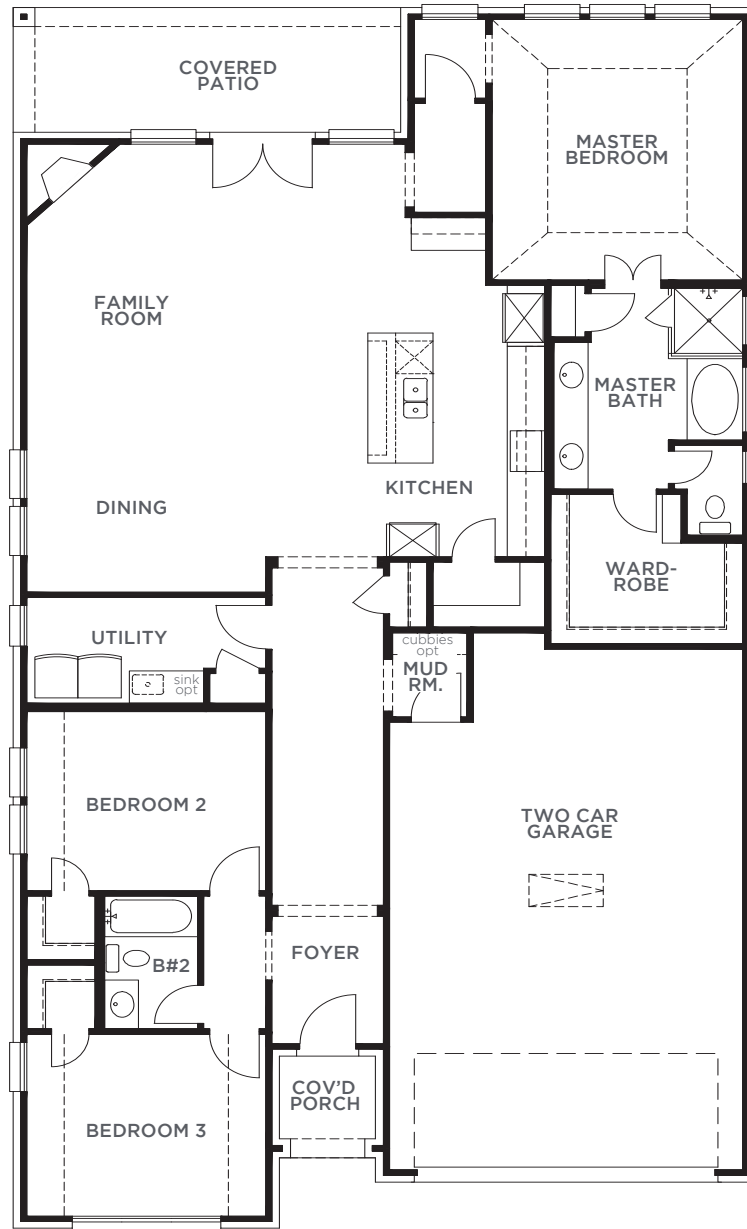
FIRST FLOOR
